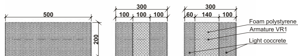
Sizes of thermoblocks
